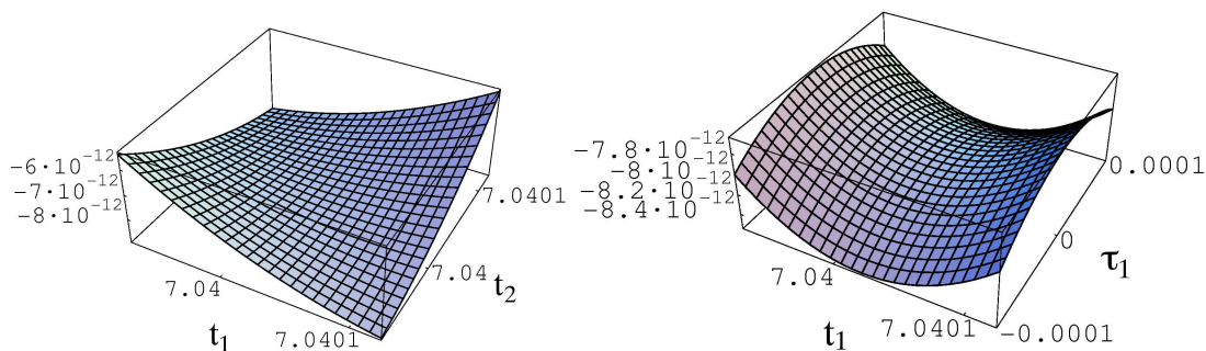
Figure 1: The non-supersymmetric vacuum for the supergravity theory specified in (4.2) for our toy example. The fields are T_1 = t_1 + i\tau_1 and T_2 = t_2 + i\tau_2 . We have plotted the potential in two slices through field space, viz., t_1-t_2 and t_1-\tau_1 . A shift in the V axis of 2.09279725 \times 10^{-3} has been performed so that the very shallow vacuum can be plotted effectively.
