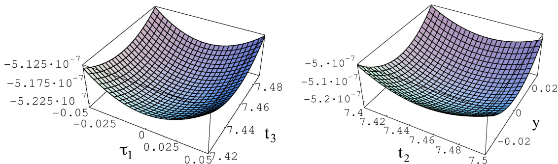
Figure 2: The non-supersymmetric extremum corresponding to the ideal I_2 in (4.11), for the supergravity potential specified in (4.10). The fields are T_i = -it_i + \tau_i and U = -ix + y ; we have here plotted the slices in (\tau_1, t_3) and (t_2, y) coordinates. A shift in the V axis of 4.07 \times 10^{-4} has been performed so that the very shallow vacuum can be plotted effectively.
